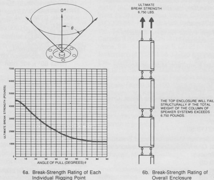
FIGURE 6 — DML-1152APF and DML-1152ACF Ultimate-Break-Strength Ratings
