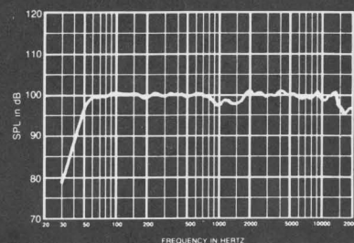
FIGURE 1 — DML-1152A/DMC-1152A Axial Frequency Response (1 watt/1 meter into LF midband)
