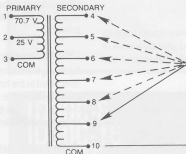
FIGURE 5 — Transformer Wiring
