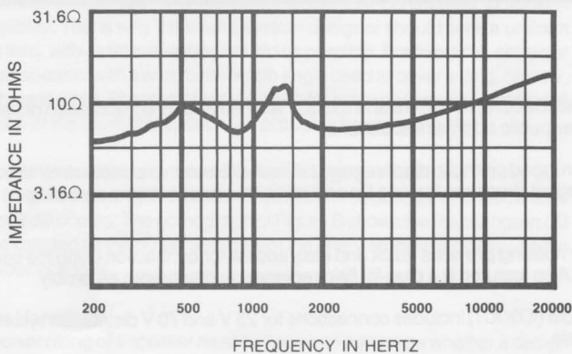
FIGURE 3 Impedance Response — Plane Wave Tube (1 inch)
