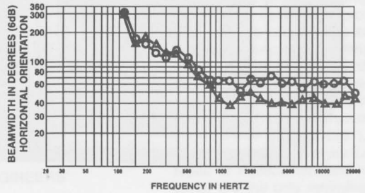
FIGURE 5 — MTH-2.5/64B Directivity vs. Frequency
