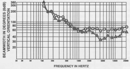
FIGURE 4 — MTH-2.5/64B Beamwidth vs. Frequency
