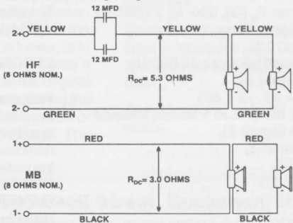
FIGURE 7 — MTH-2.5/64B Wiring Diagram
