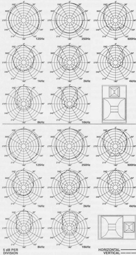
FIGURE 3 — MTH-2.5/64B Polar Response
