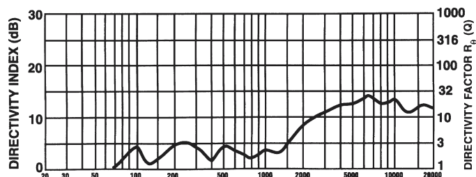
Directivity
