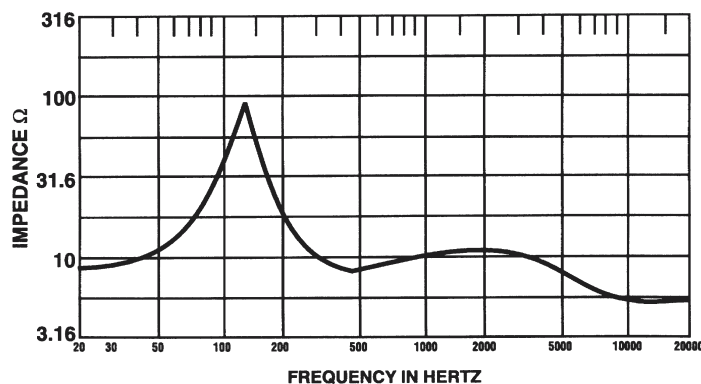
Impedance Response
