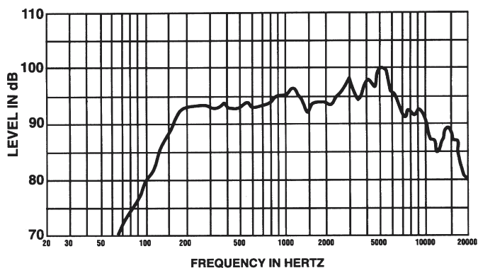
Frequency Response
