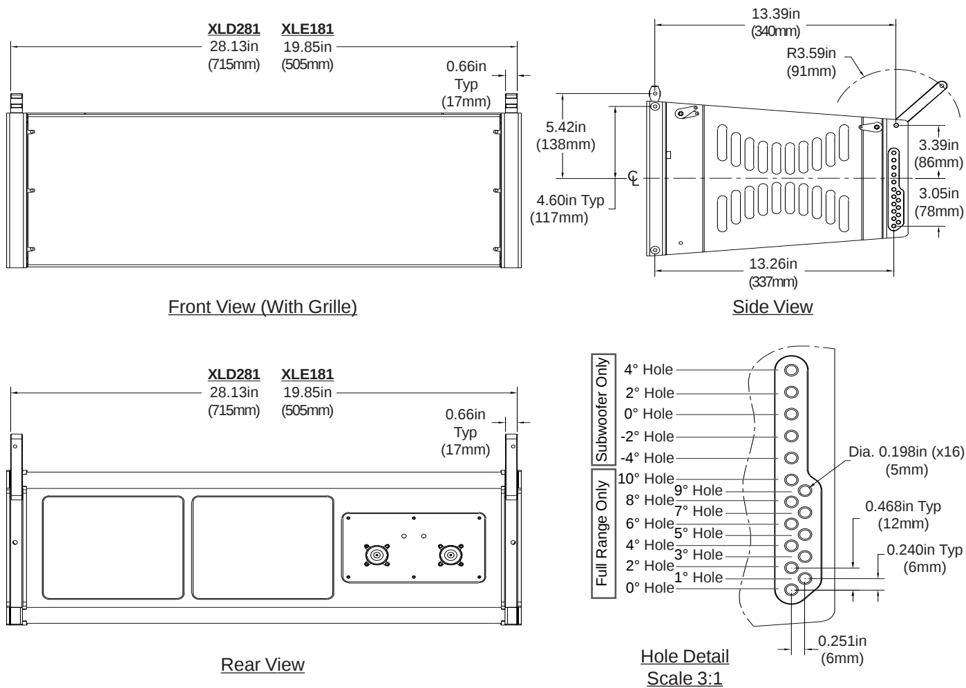
Figure 4a: XLD281 and XLE181 Rigging Dimensions
