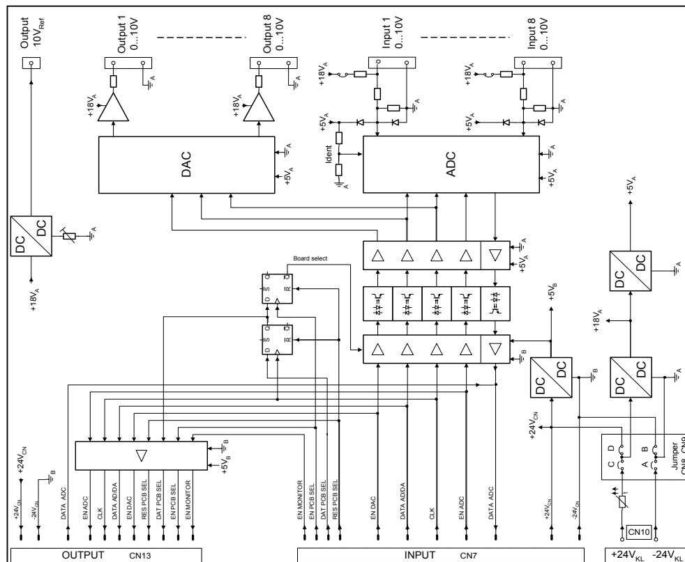
DCS416 Block Diagram
