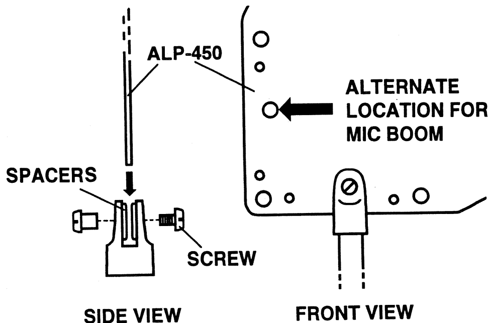
Figure 2 Microphone Stand Adaptor
