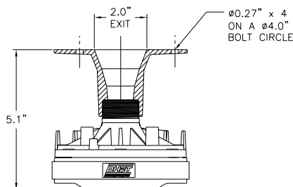
Side View (Shown with Optional ADH-5 Adapter)
