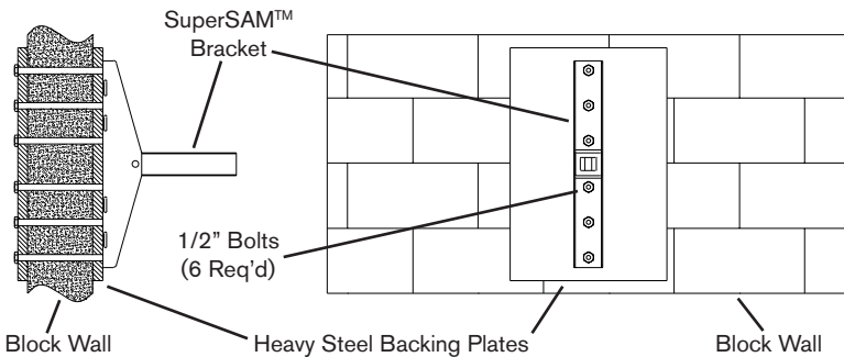
Figure 3: Block Wall Mounting
