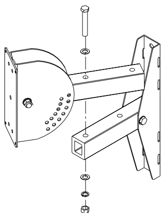
Exploded View
