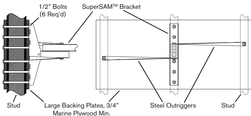
Figure 4: Stud Mounting
