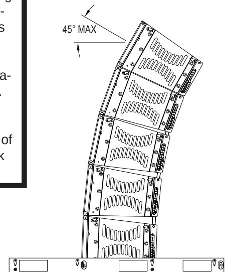
Figure 7: Single Stack - XLE181 at Middle (5 Max)
