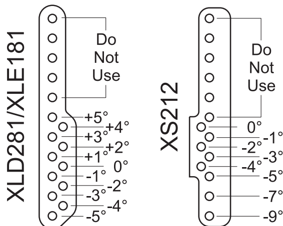
Figure 2: Angle Instruction for Bottom Enclosure Pin Position
