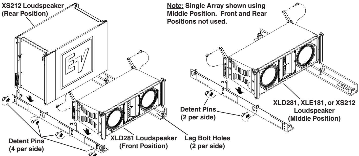
Figure 1: Attaching Loudspeakers to Groundstack Rails
