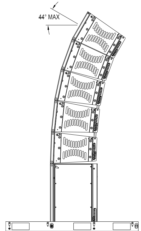
Figure 5: Single Stack - XLD281 (5 Max) and XS212 (1 Max) Combination Array at Middle
