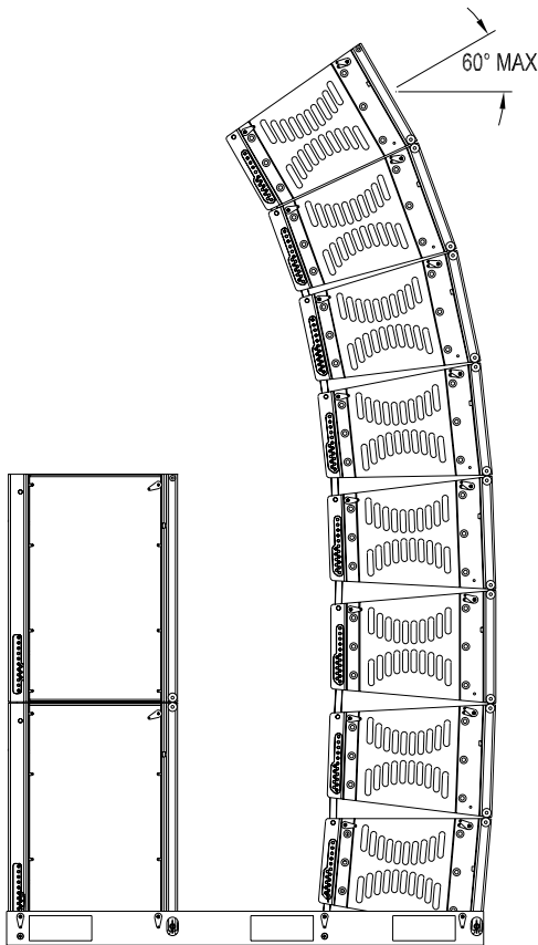
Figure 3: Dual Stack - XLD281 Array at Front (8 Max) XS212 Array at Rear (2 Max)
