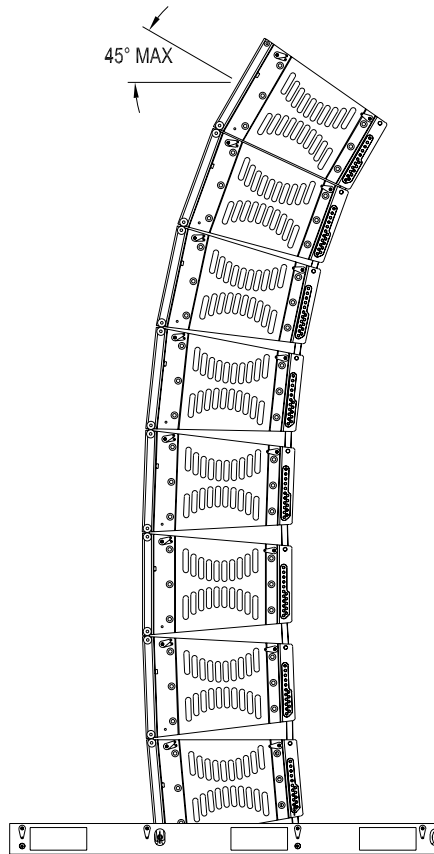
Figure 4: Single Stack - XLD281 Array at Middle (8 Max)
