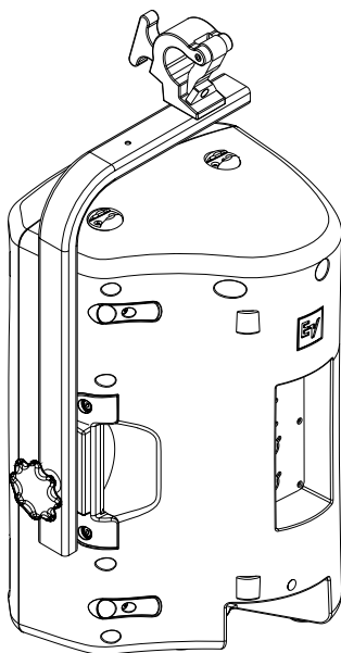
Fully Assembled with HA-3 Handle Mount and VSA-1 Strong-Arm Mount
