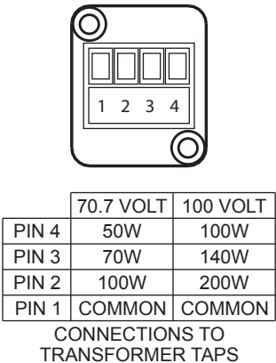
Sx300PIX Connection
