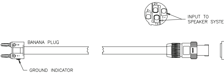
Sx300PI Connection
