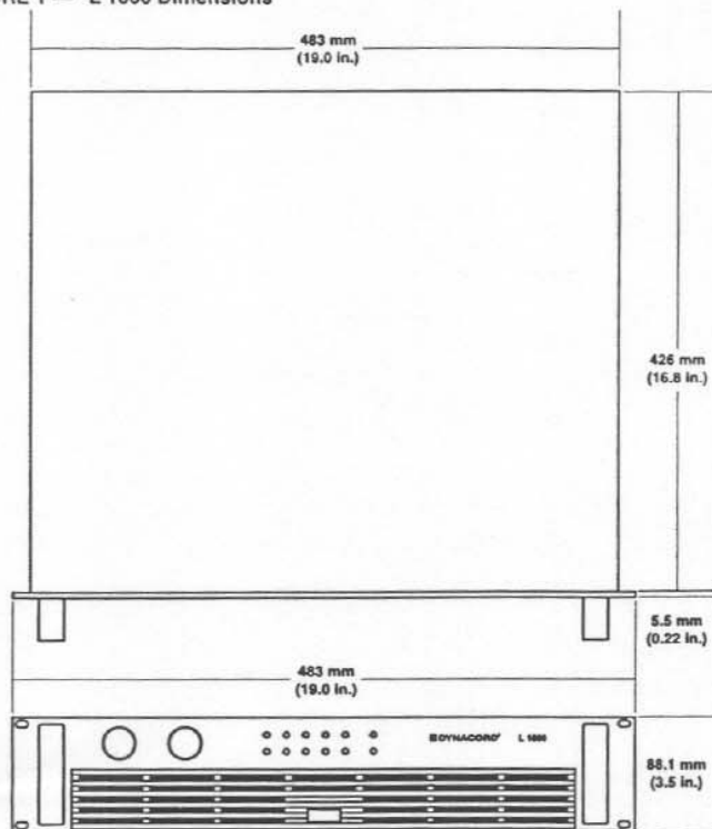
FIGURE 1 — L 1000 Dimensions
