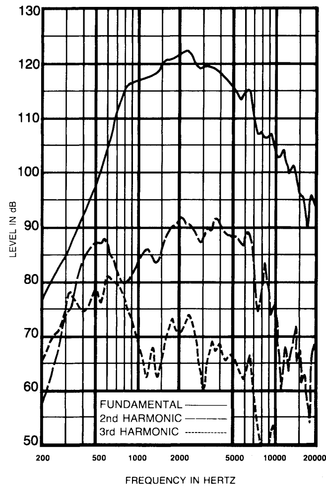
FIGURE 5 Distortion Response — DH1506 Driver on HT94 Horn (2 Watts/1 Meter)
