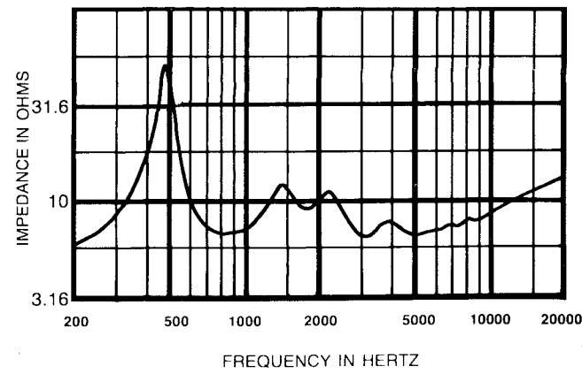
FIGURE 7 Impedance Response — DH1506 on HT94 Horn
