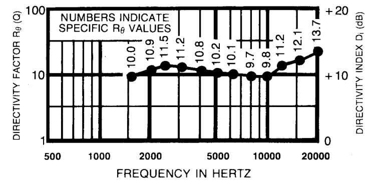
FIGURE 2 Directivity vs Frequency — HT94 Whole Space (Anechoic)
