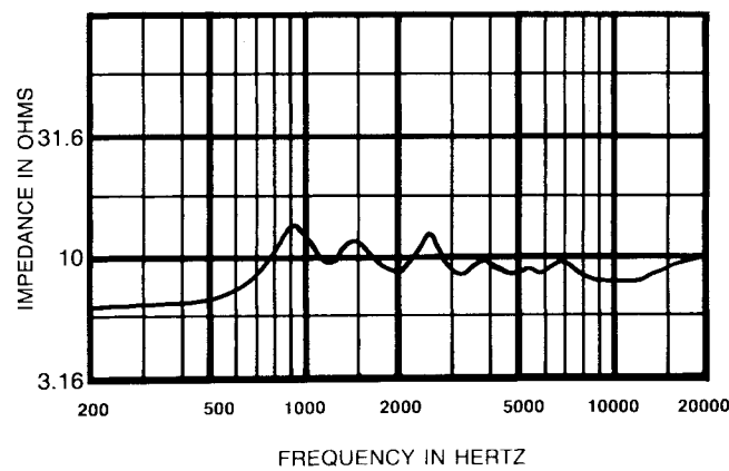
FIGURE 6 Impedance Response — DH2305 on HT94 Horn
