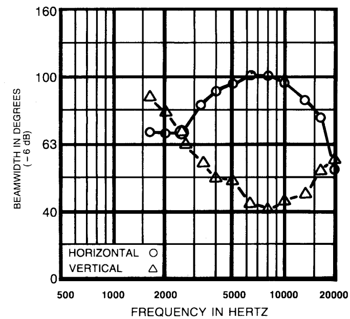
FIGURE 3 Beamwidth vs Frequency — HT94 Whole Space (Anechoic)
