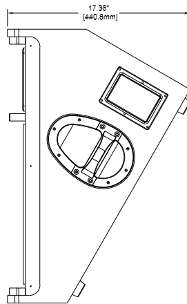
Right View
