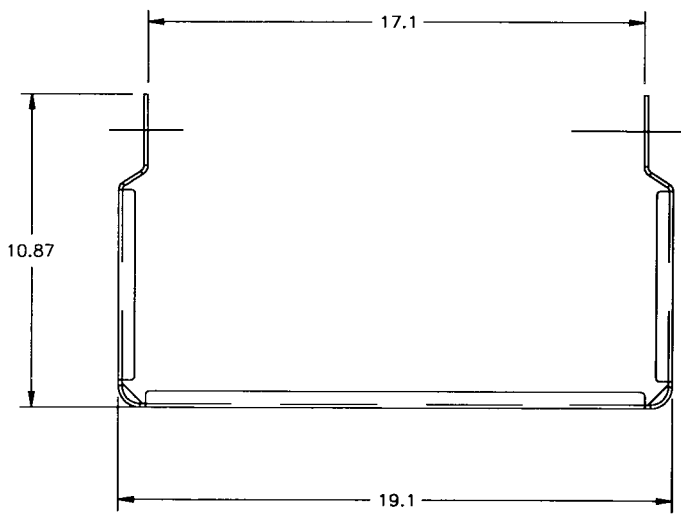
Figure 3—MB-VI15 Mounting Bracket
