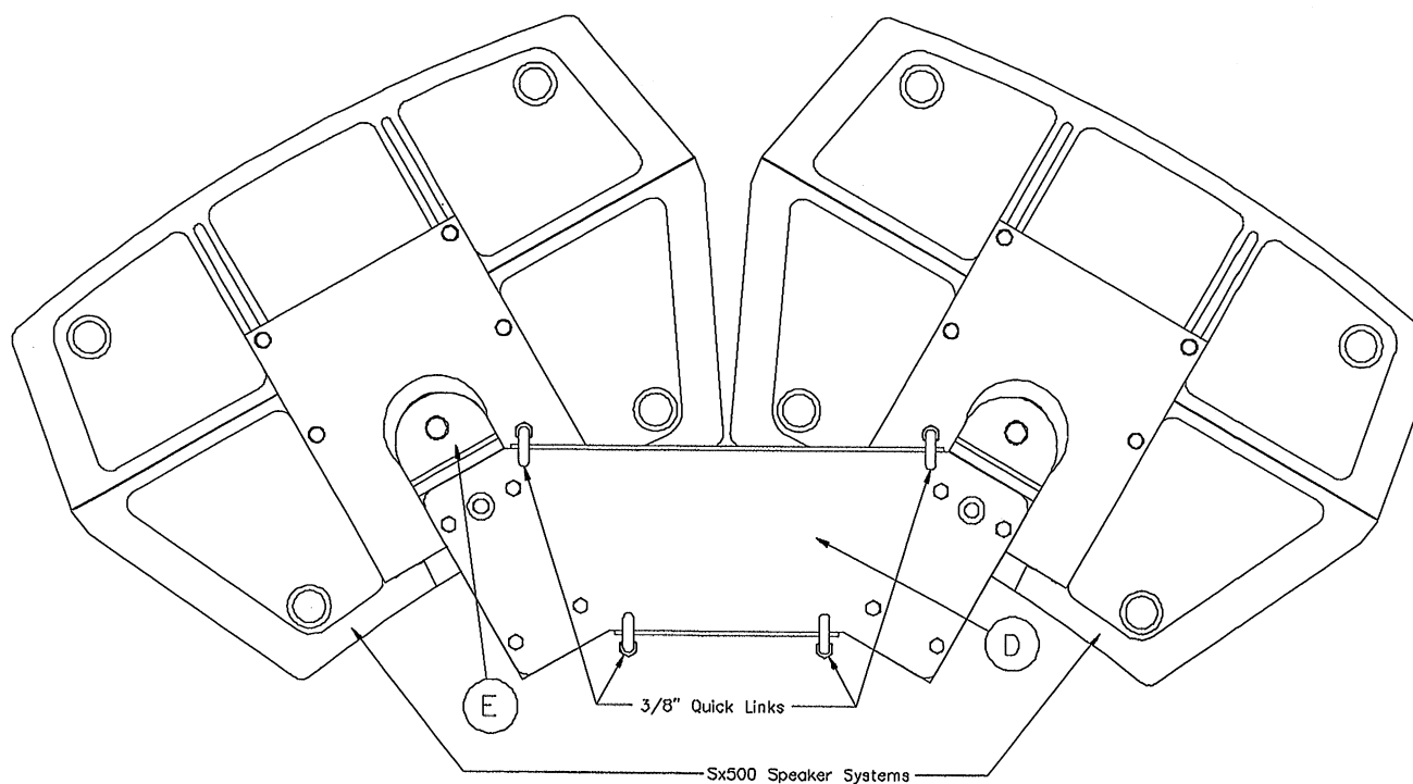
Figure 2B—Two-Speaker Horizontal Array using Mb600 and Mb500 Brackets
