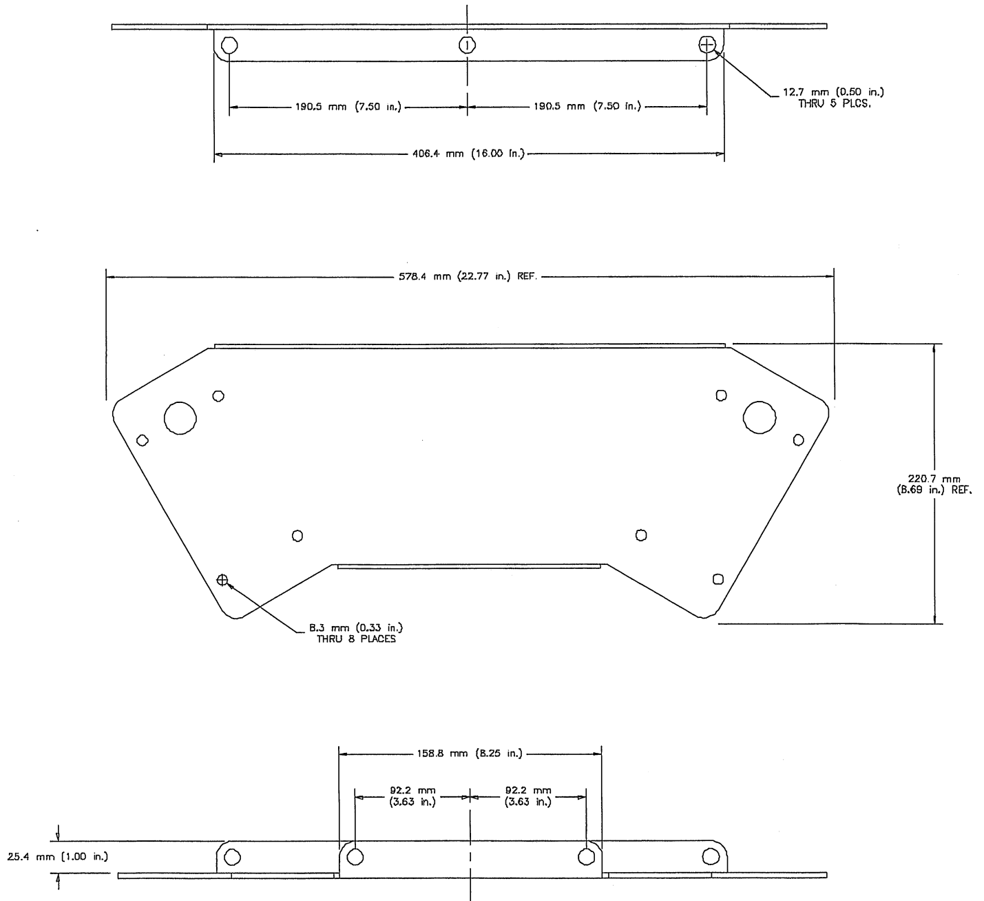
Figure 1—Mb600 Horizontal Array Kit
