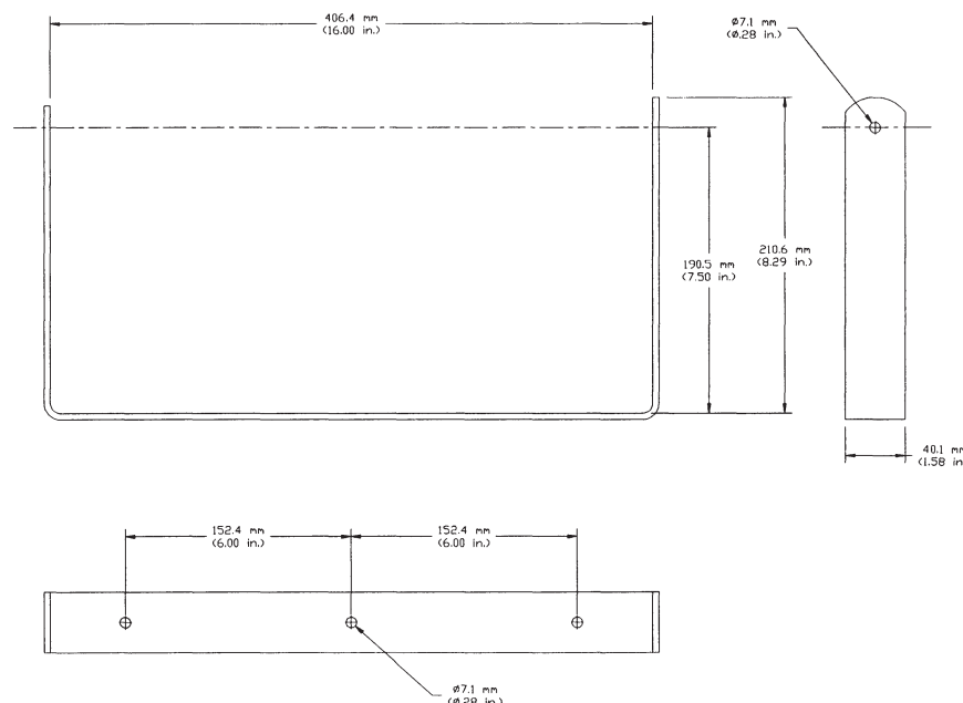
Figure 2—Sx80MB Mounting Bracket Dimension
