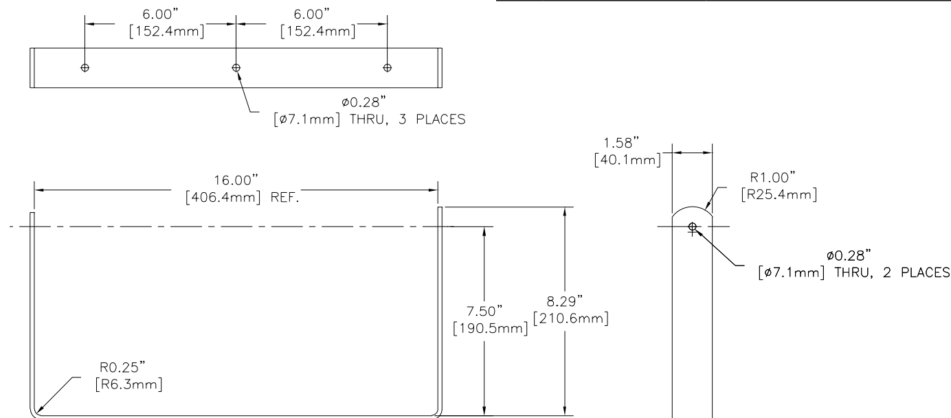
Fig. 2 - Sx80SMB Mounting Bracket Dimensions
