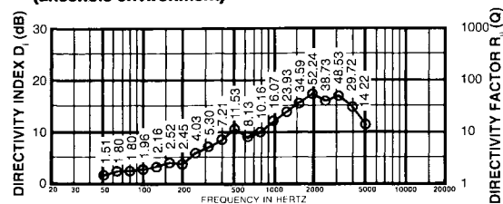
FIGURE 4 — TL550D One-Third-Octave Directivity vs Frequency (anechoic environment)
