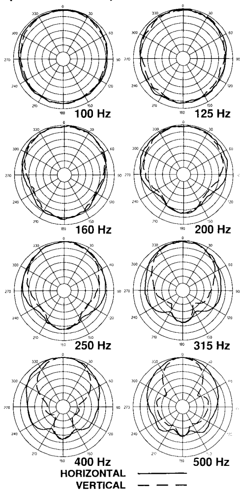
FIGURE 2 — TL550D One-Third-Octave Polar Responses (anechoic environment)
