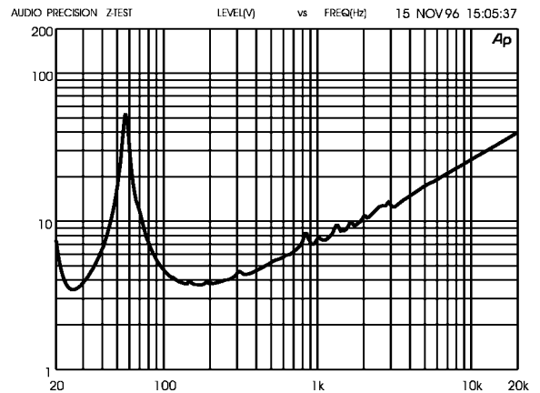
FIGURE 6 — TL770D Impedance
