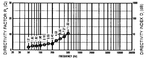
FIGURE 4 — TL770D One-Third-Octave Directivity vs Frequency (anechoic environment)
