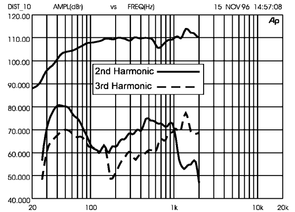
FIGURE 5 — TL770D Harmonic Distortion, 0.1 Rated Power Input (80 watts), 10 Feet on Axis
