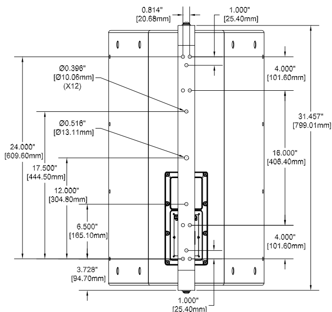
Figure 9: EVF-UB Rear View Dimensions
