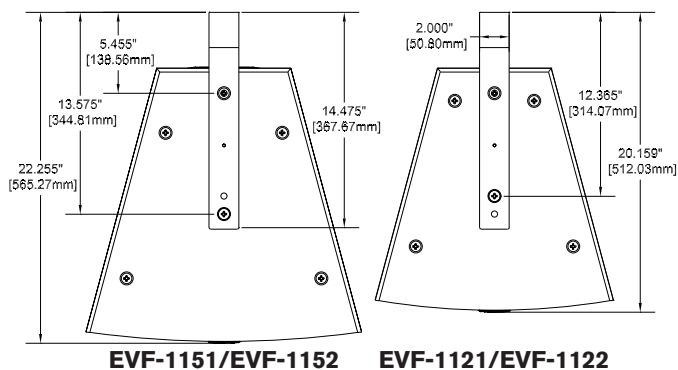
Figure 8: EVF-UB Top View Dimensions
