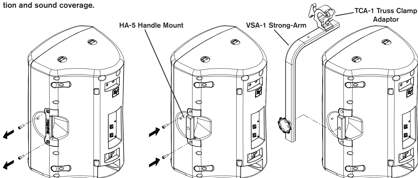
Step 1: Remove Handle Bolts and Handle
