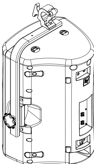
Step 1: Remove Handle Bolts and Handle
