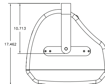
MB5 Top View Dimensions
