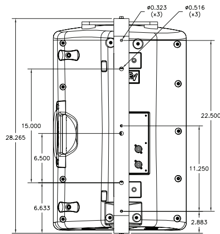
MB5 Rear View Dimensions
