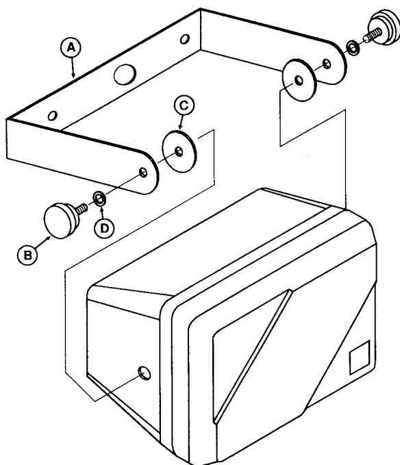
FIGURE 1 Wall Mounting
