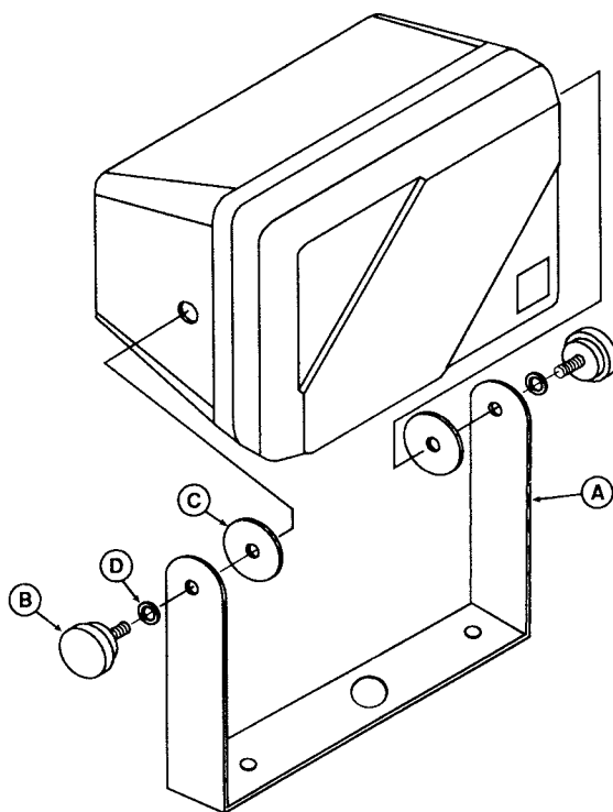
FIGURE 2 Stand Mounting
