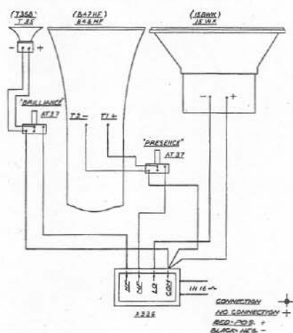
Fig. 4 — Schematic Wiring Diagram Indirect Radiator 4-way System
