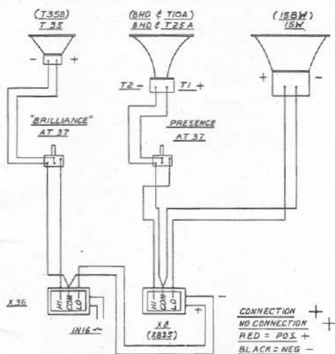
Fig. 3 — Schematic Wiring Diagram Separate 3-way System
