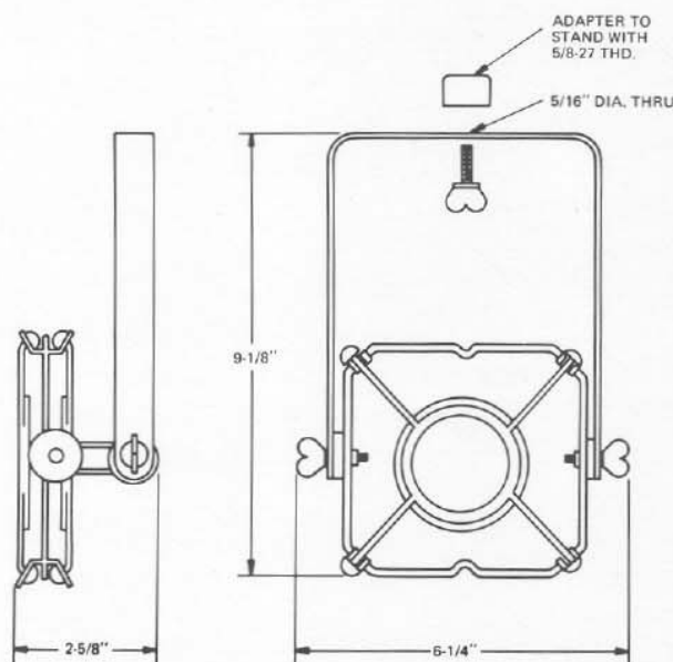
Figure 1 — Dimensions
