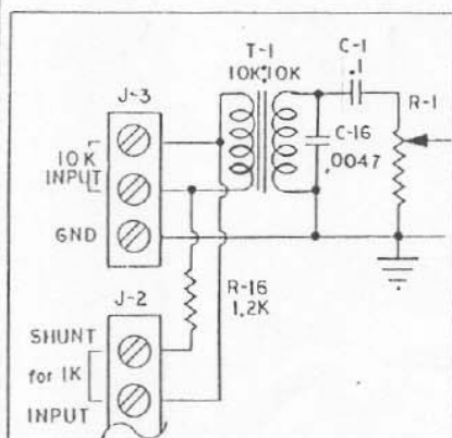
ALTERNATE INPUT CIRCUIT USED ON MODEL 582
