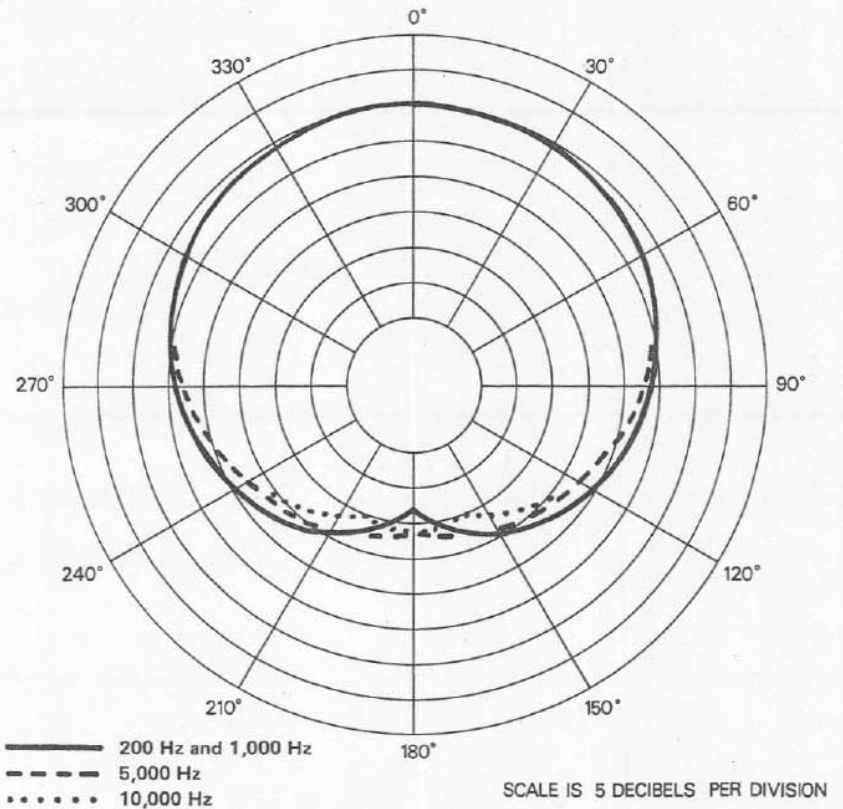
FIGURE 4 — Polar Response
