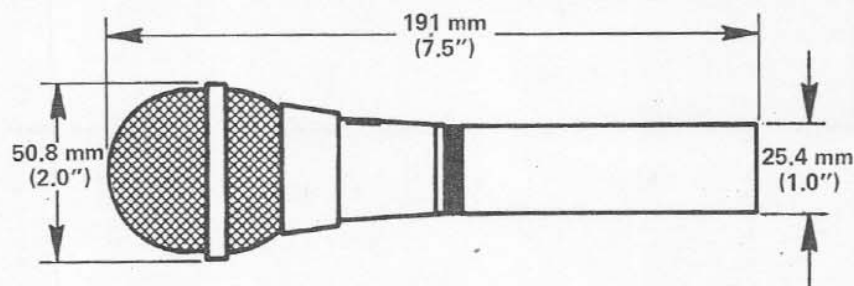
FIGURE 1 – Dimensions
