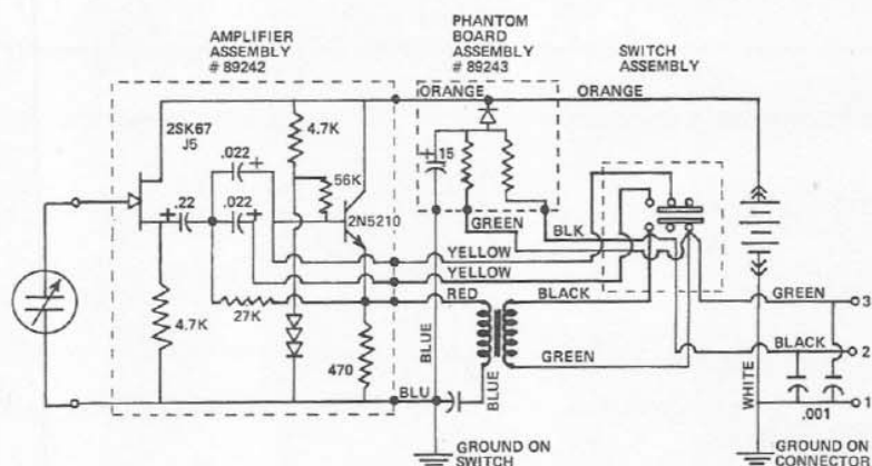
FIGURE 2 – Wiring Diagram
