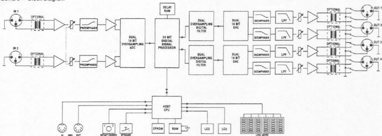
FIGURE 3 — Block Diagram
