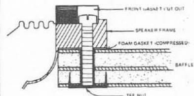
FIGURE 9 Front Mounting Detail (Not to scale)
