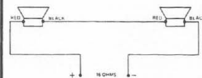
FIGURE 12 Connection of 2 EVM-10M Speakers in Series
