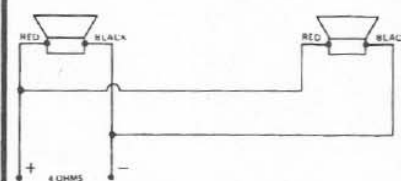
FIGURE 11 Connection of 2 EVM-10M Speakers in Parallel
