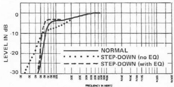
FIGURE 6 TL806/EVM-12S Low Frequency Response
