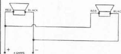
FIGURE 11 Connection of 2 EVM-12S Speakers in Parallel
