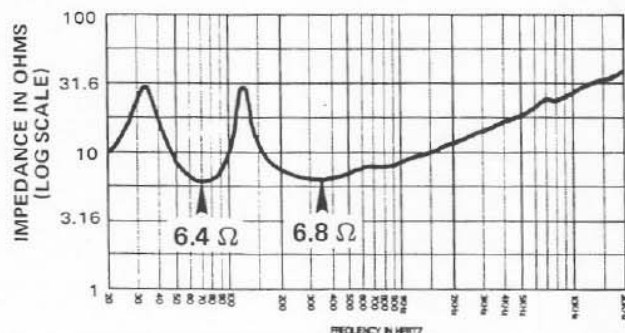
FIGURE 8 TL806/EVM-12S Input Impedance vs. Frequency
