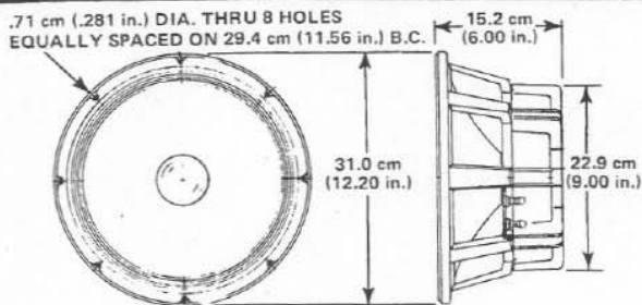
FIGURE 1 – Dimensions
