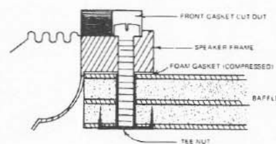
FIGURE 9 Front Mounting Detail (Not to Scale)
