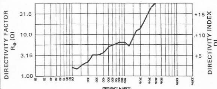
FIGURE 5 TL806/EVM-12S Directivity Factor and Directivity Index vs. Frequency
