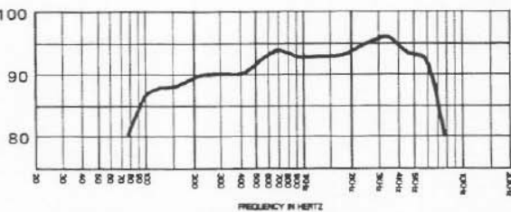
FIGURE 2 – TL806/EVM-12S Frequency Response (Swept 1/3-Octave Band Pink Noise, 4 V at 10 ft. on Axis, Half-Space Environment)
