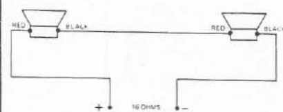
FIGURE 12 Connection of 2 EVM-12S Speakers in Series
