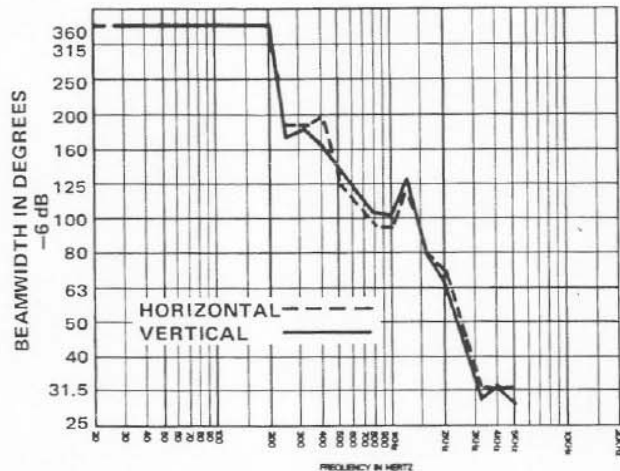
FIGURE 4 TL806/EVM-12S Beamwidth vs. Frequency
