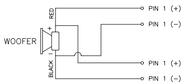
SCHEMATIC DIAGRAM
