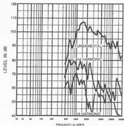
FIGURE 3 MIS4C/MIS8C Frequency Response (1 watt at 1 meter)
