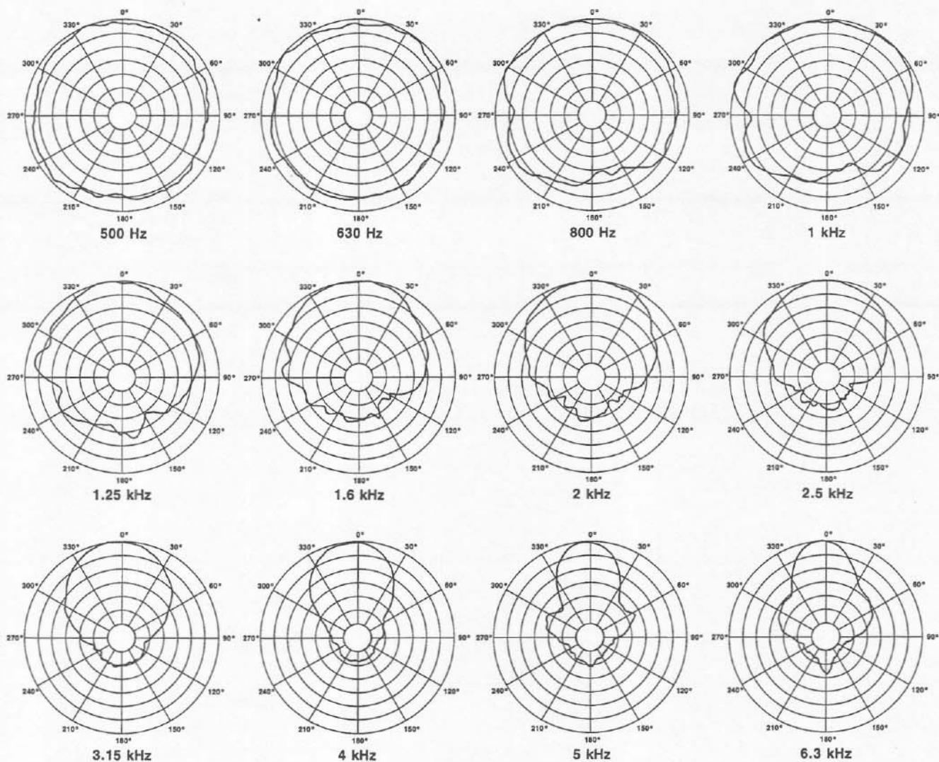
FIGURE 1 MIS4C/MIS8C Polar Response
