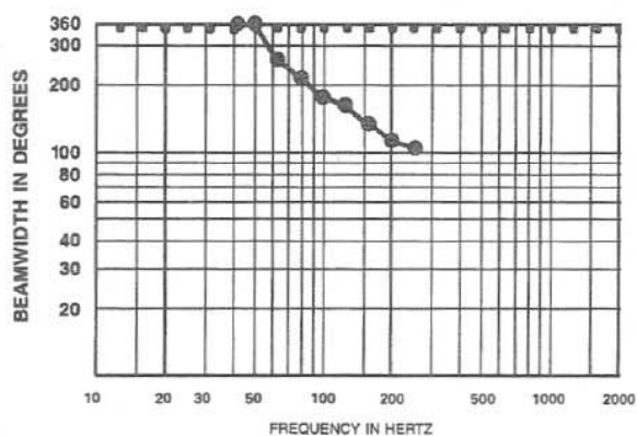
FIGURE 3 MTL-4 Beamwidth vs. Frequency
