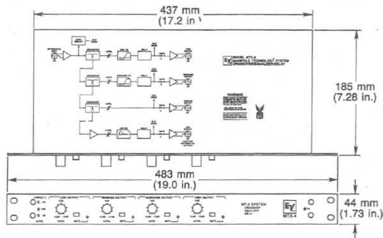
FIGURE 1 — Dimensions
