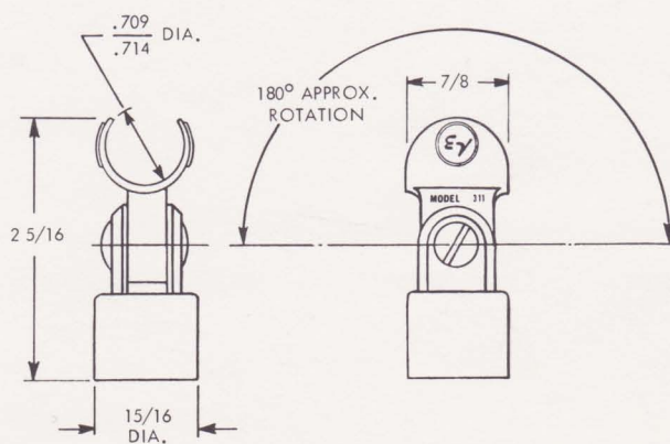
Figure 2-Dimensions-311
