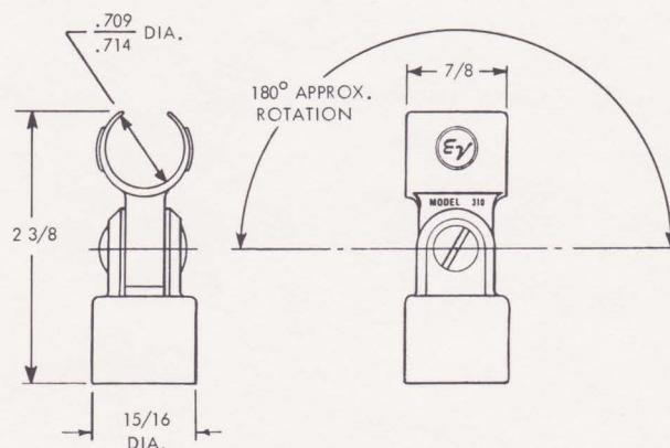
Figure 1-Dimensions-310
