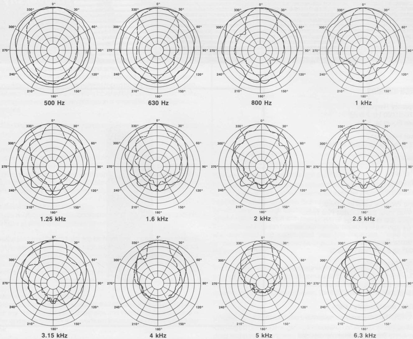
FIGURE 1 LR2SA Polar Response
