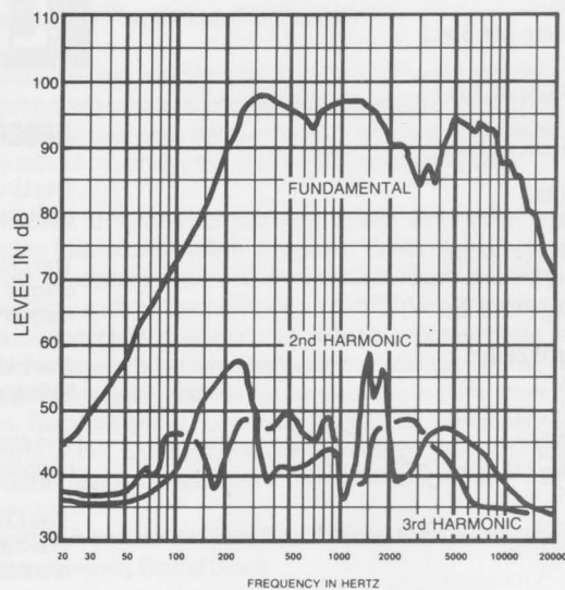
FIGURE 3 LR2SA Frequency Response (1 watt at 1 meter)
