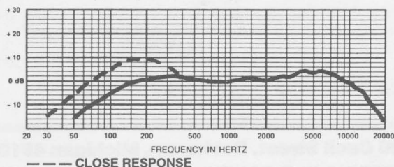
FIGURE 1 — Frequency Response
