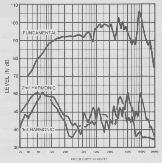
FIGURE 3 MC8A Frequency Response (1 watt at 1 meter)
