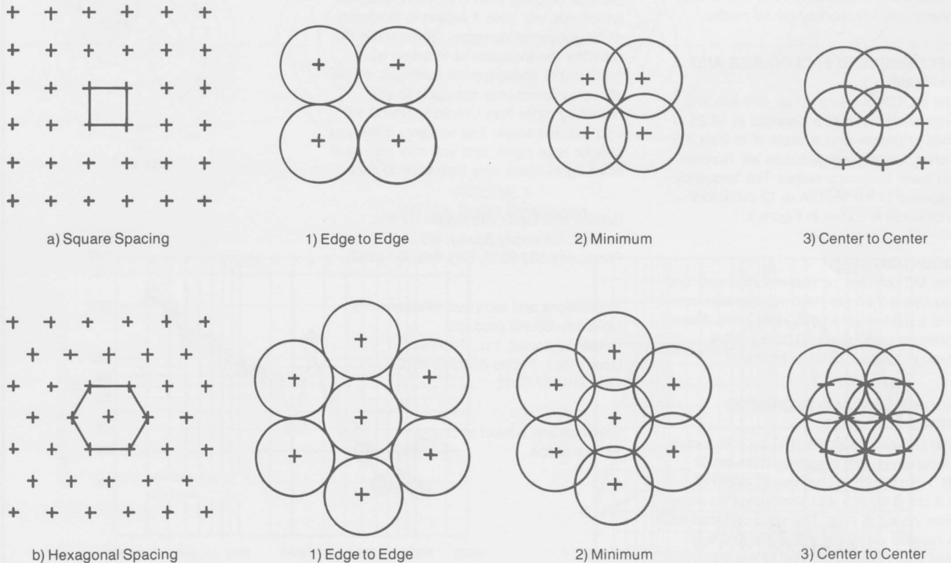
FIGURE A — Basic Ceiling Speaker Patterns
