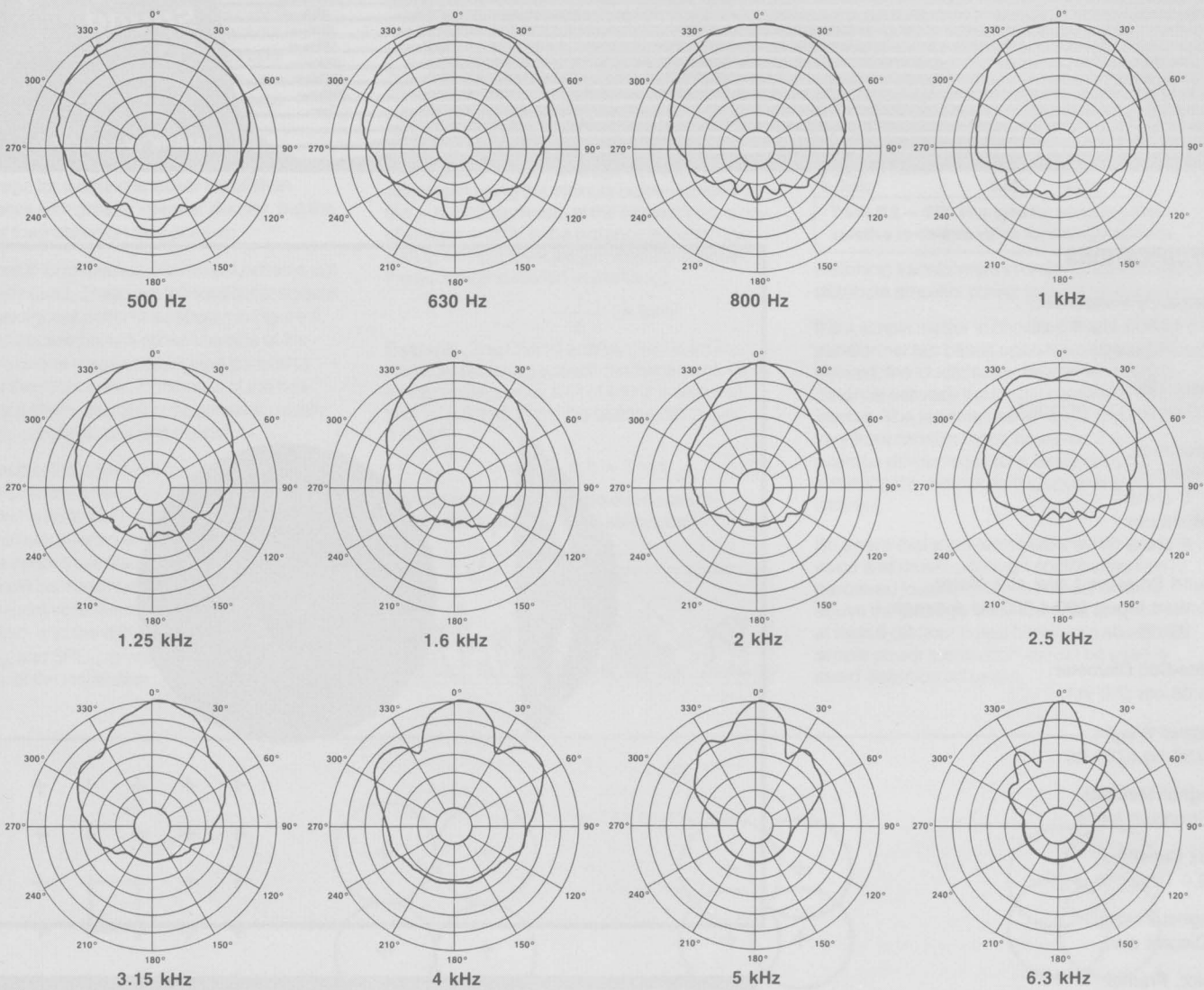
FIGURE 1 MC12A Polar Response
