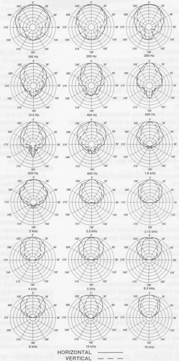
FIGURE 8 — Polar Response
