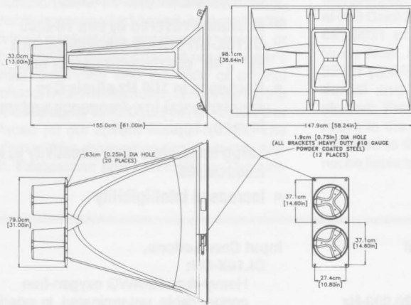
FIGURE 3 — Dimensions
