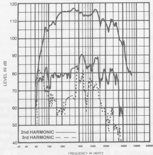
FIGURE 5 — Distortion Response, 10% Power
