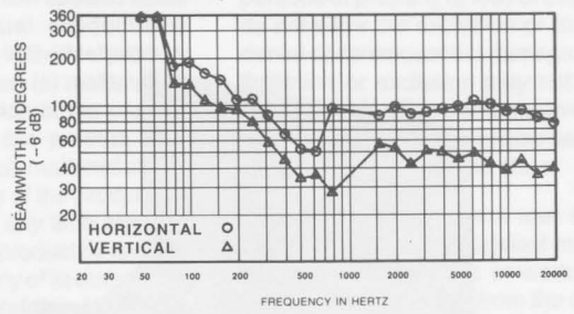
FIGURE 6 — Beamwidth Response
