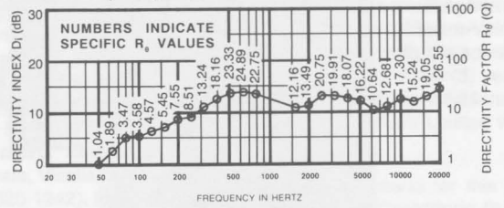
FIGURE 7 — Directivity Response
