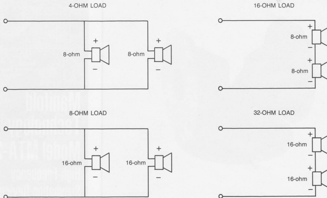
FIGURE 2 Electrical Connections
