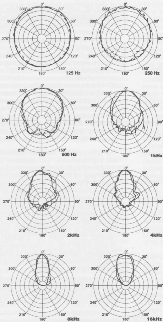
FIGURE 3 — MTH-2.5/22BT Polar Response
