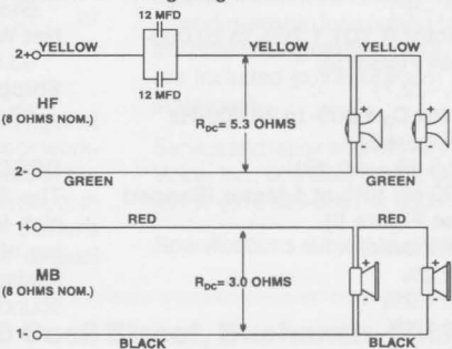
FIGURE 7 — MTH-2.5/22BT Wiring Diagram
