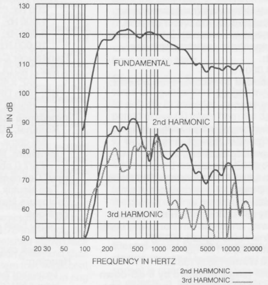
FIGURE 6 — MTH-2.5/22BT Harmonic Distortion
