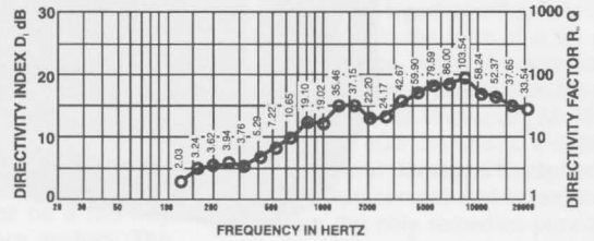
FIGURE 5 — MTH-2.5/22BT Directivity vs. Frequency
