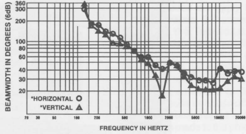
FIGURE 4 — MTH-2.5/22BT Beamwidth vs. Frequency
