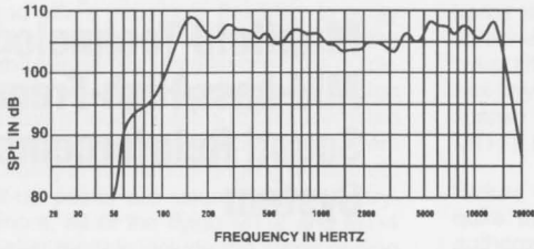
FIGURE 1 — MTH-2.5/22BT Axial Frequency Response
