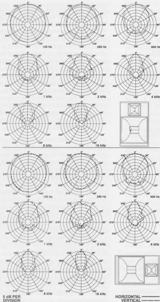
FIGURE 3 — Polar Response
