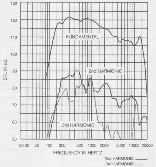
FIGURE 6 — Harmonic Distortion
