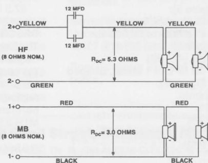
FIGURE 7 — Wiring Diagram
