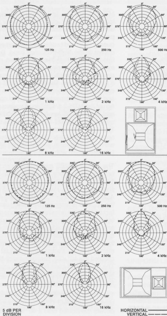
FIGURE 3 — Polar Response
