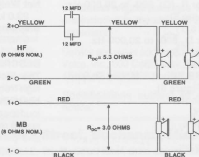
FIGURE 7 — Wiring Diagram
