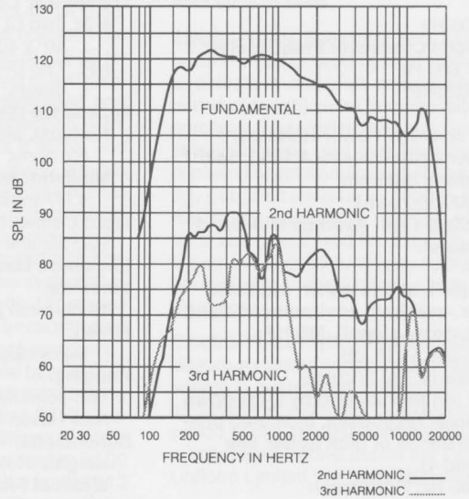
FIGURE 6 — Harmonic Distortion
