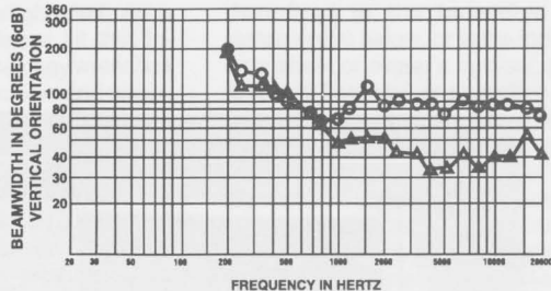
FIGURE 4 — MTH-2.5/94B Beamwidth vs. Frequency
