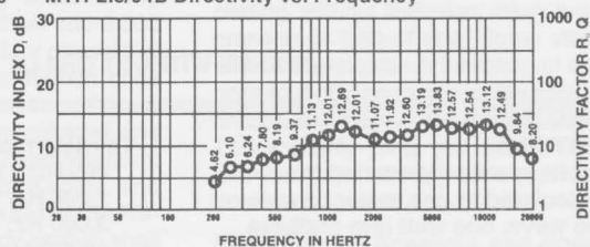
FIGURE 5 — MTH-2.5/94B Directivity vs. Frequency
