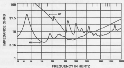
FIGURE 2 — MTH-2.5/94B Impedance vs. Frequency
