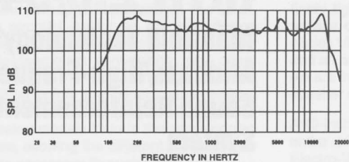
FIGURE 1 — MTH-2.5/94B Axial Frequency Response
