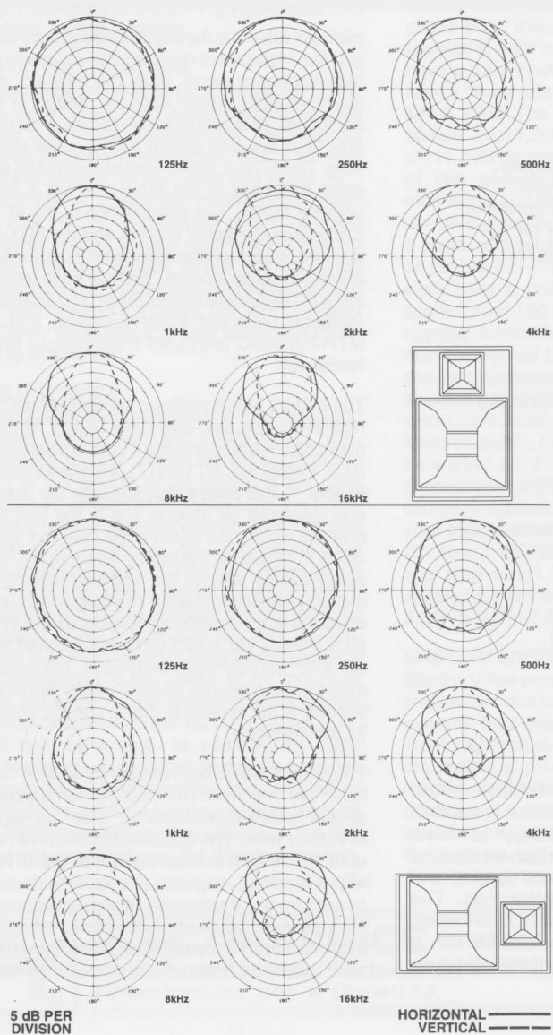
FIGURE 3 — MTH-2.5/94B Polar Response
