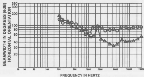
FIGURE 5 — MTH-2.5/94B Directivity vs. Frequency
