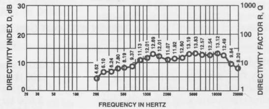
FIGURE 5 — MTH-2.5/94BT Directivity vs. Frequency
