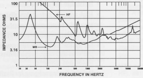
FIGURE 2 — MTH-2.5/94BT Impedance vs. Frequency
