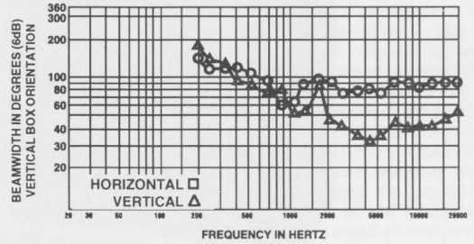
FIGURE 5 — MTH-2.5/94BT Directivity vs. Frequency
