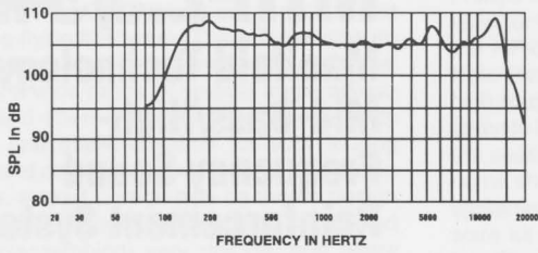
FIGURE 1 — MTH-2.5/94BT Axial Frequency Response
