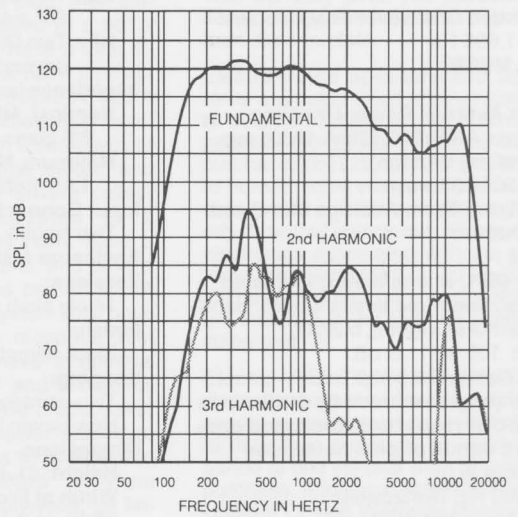
FIGURE 6 — MTH-2.5/94BT Harmonic Distortion
