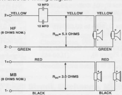
FIGURE 7 — MTH-2.5/94BT Wiring Diagram
