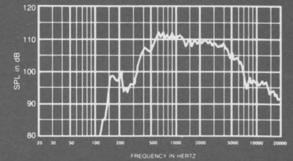
FIGURE 1 Axial Frequency Response 1 Watt/1 Meter
