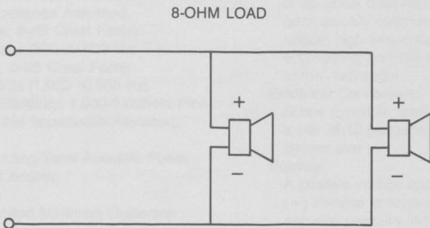
FIGURE 8 Electrical Connections
