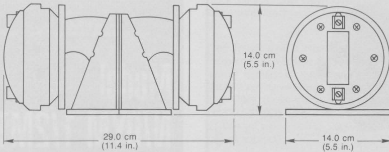
FIGURE 2 Dimensions
