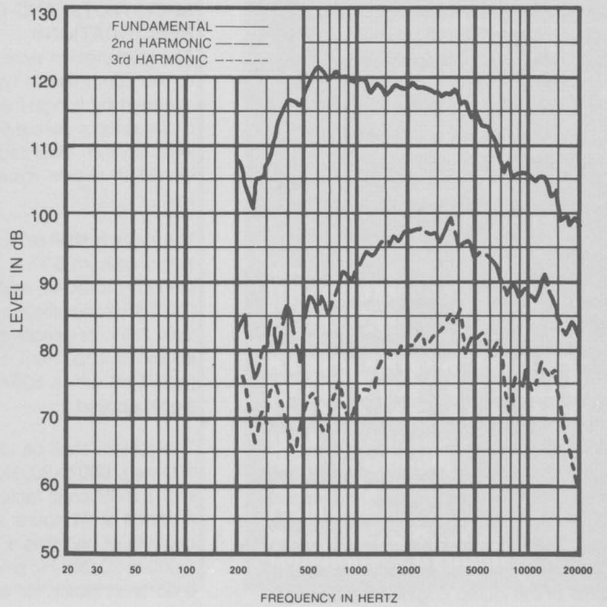
FIGURE 5 Distortion Response, HP9040 Horn, 10 Watts/1 Meter
