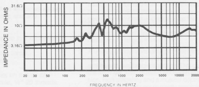
FIGURE 9 Impedance Response — HP9040 Horn 16-Ohm Driver
